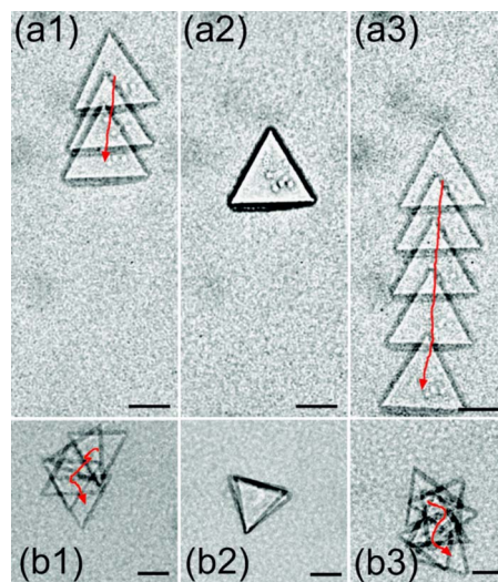
FIG. 2. (Color online) Phototactic control of a 50 \mu\text{m} triangular microstructure: (a1) translation with the average velocity of 9.15 \mu\text{m/s} before UV exposure, (a2) during 5 s exposure translation stops, (a3) after exposure translation fully resumes within 8 s, and (b1) rotation with the average angular velocity of 1.05 rad/s on swarm plate before UV exposure; centroid follows path shown (b2) rotation stops during 5 s exposure and (b3) rotation fully resumes within 7 s after exposure. The scale bars are 25 \mu\text{m} .
