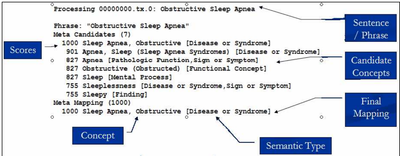
Figure 5: MetaMap Transfer Output (United States National Library of Medicine, 2005b)
