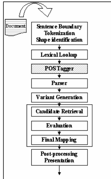
Figure 4 – UMLS MetaMap Transfer process (United States National Library of Medicine, 2005b)
